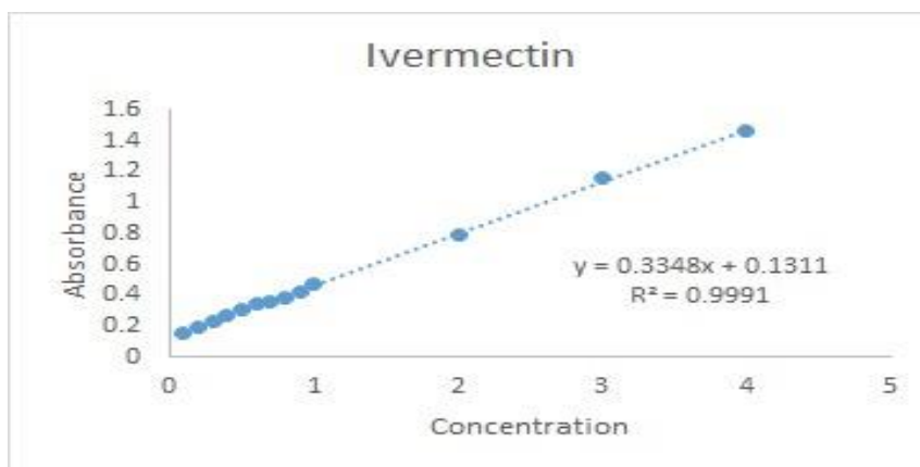
Figure 5. Calibration plot of Ivermectin
