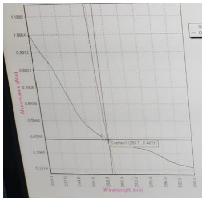
Figure 3. The Isobestic Point was established at the \lambda_{\max} 260.7 showing absorbance 0.4819
